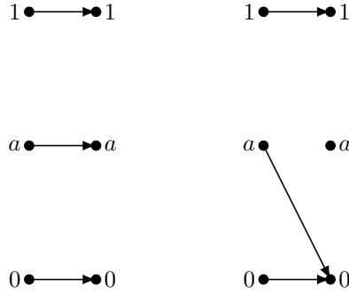
FIGURE 9. The two possible exponentiations x \mapsto x^a
