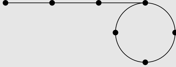
FIGURE 2. \mathbb{N}_{3,4}
