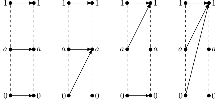
FIGURE 8. The four possible exponentiations x \mapsto x^a
