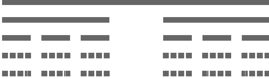
FIGURE 5. \widehat{\mathbb{Z}} as limits of \mathbb{Z}/n!\mathbb{Z}
