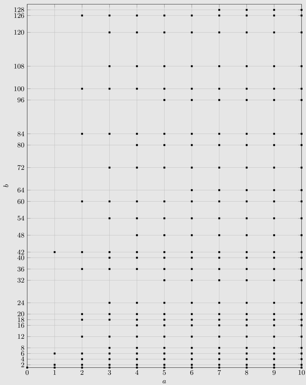
FIGURE 3. Finite quotient riels of \mathbb{N} for small a and b
