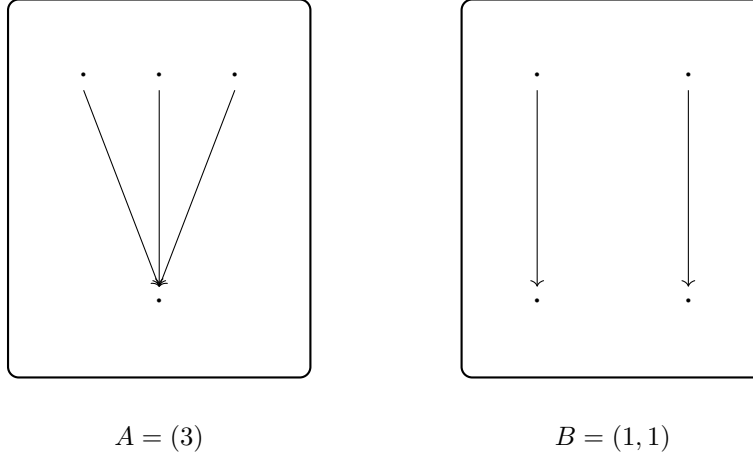
FIGURE 7. The representing object of sum-of-cubes and square-of-sum in \mathbf{FinSet}^{\rightarrow}
