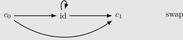
FIGURE 6. The exponential graph \rightarrow^{\rightarrow}
